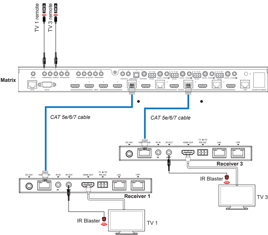
Figure 1: IR connection diagram (Matrix end)
