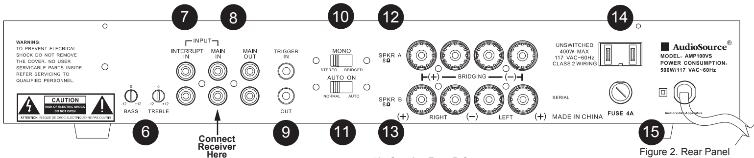
Figure 2. Rear Panel
