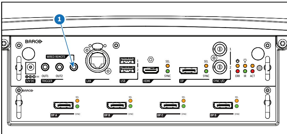
Image 3–10 RCU hardwired connection
