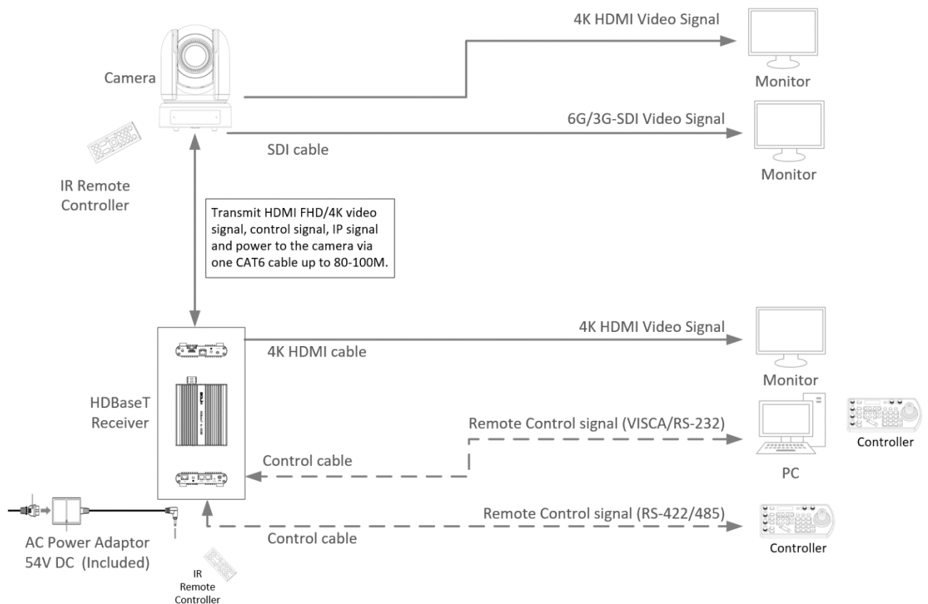
Camera Connection using HDBaseT
