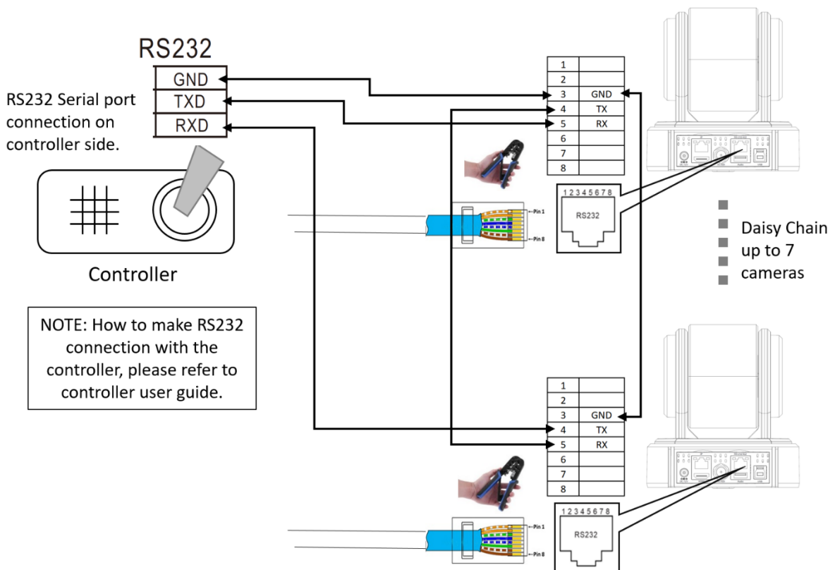
RS232 Connection with standard RS232 Serial Port PTZ Keyboard Controller
