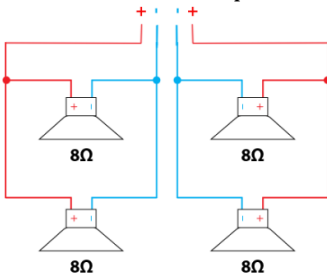
Example showing four 8 \Omega speakers
