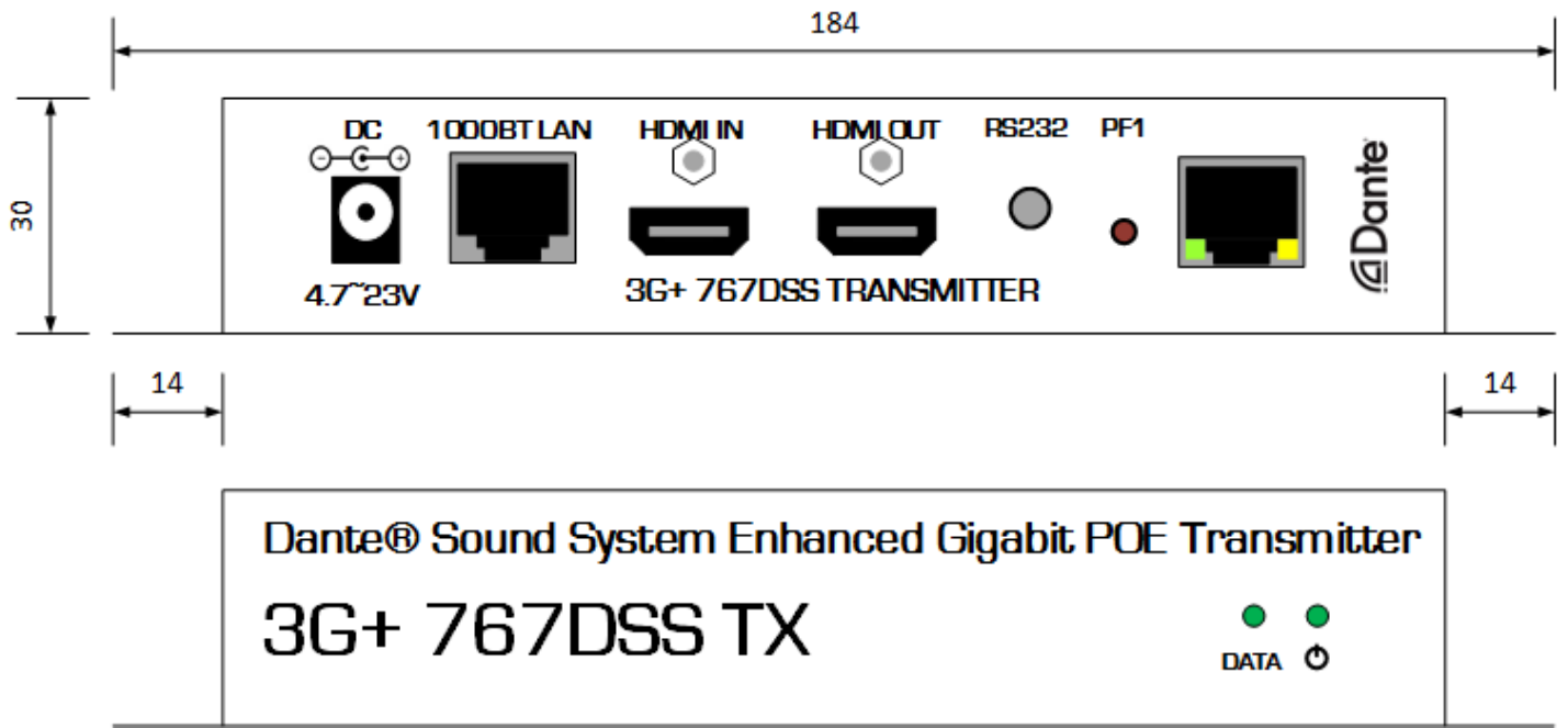
767DSS Front/Back
