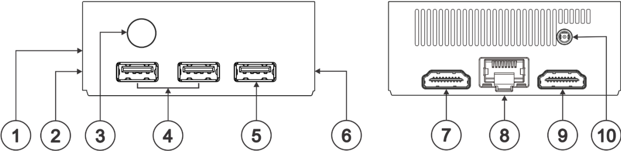
Figure 4: VIA Connect 2 Front Panel
