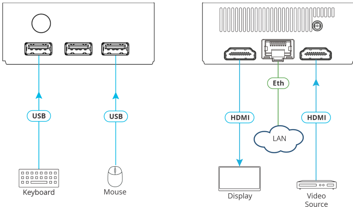
Figure 5: Connecting VIA Connect 2
