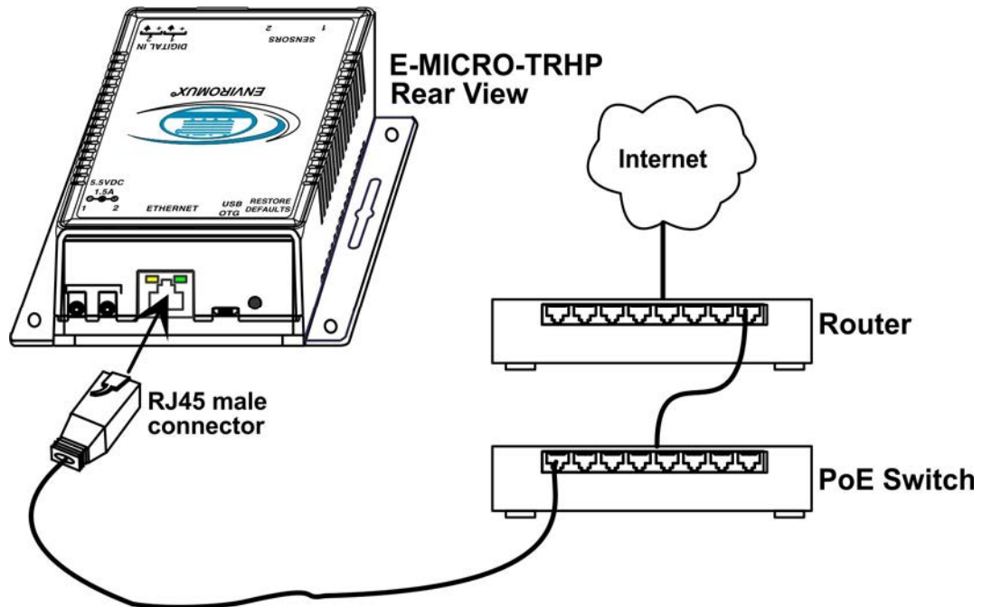
Figure 6- Connect E-MICRO to the Ethernet
