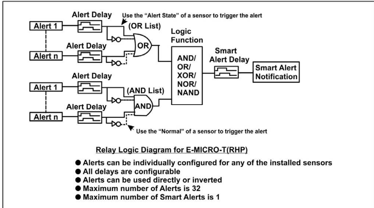
Figure 23- Event Logical Function Diagram
