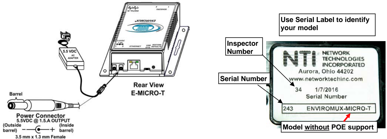
Figure 7- Connect the AC adapter and power-up
