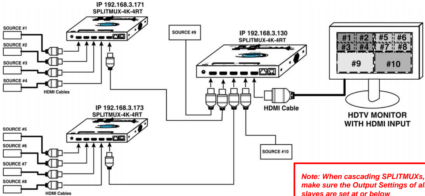
Figure 28- Cascading SPLITMUXs
