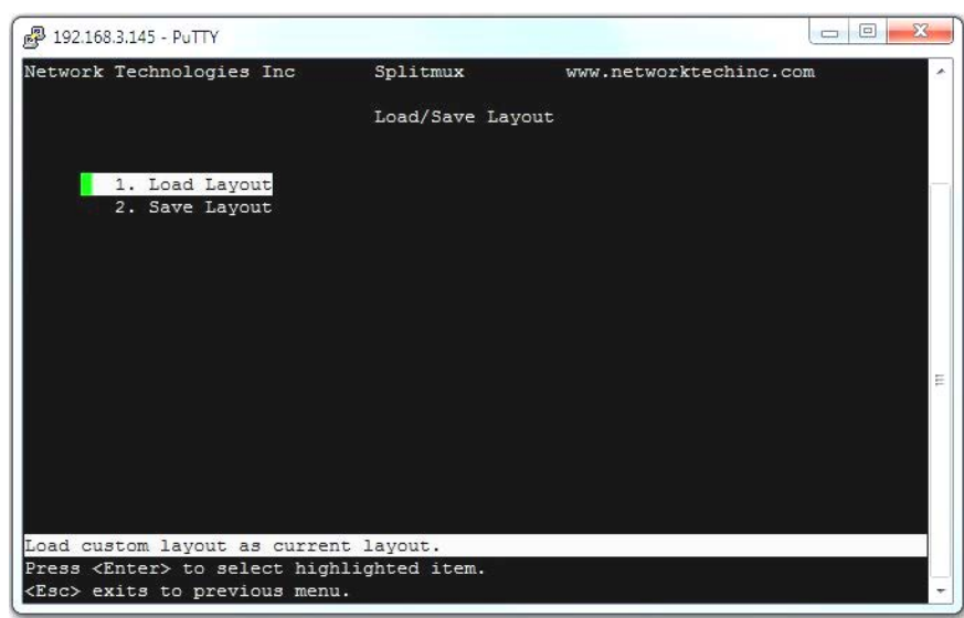
Figure 72- Text Menu- Load/Save Layout
