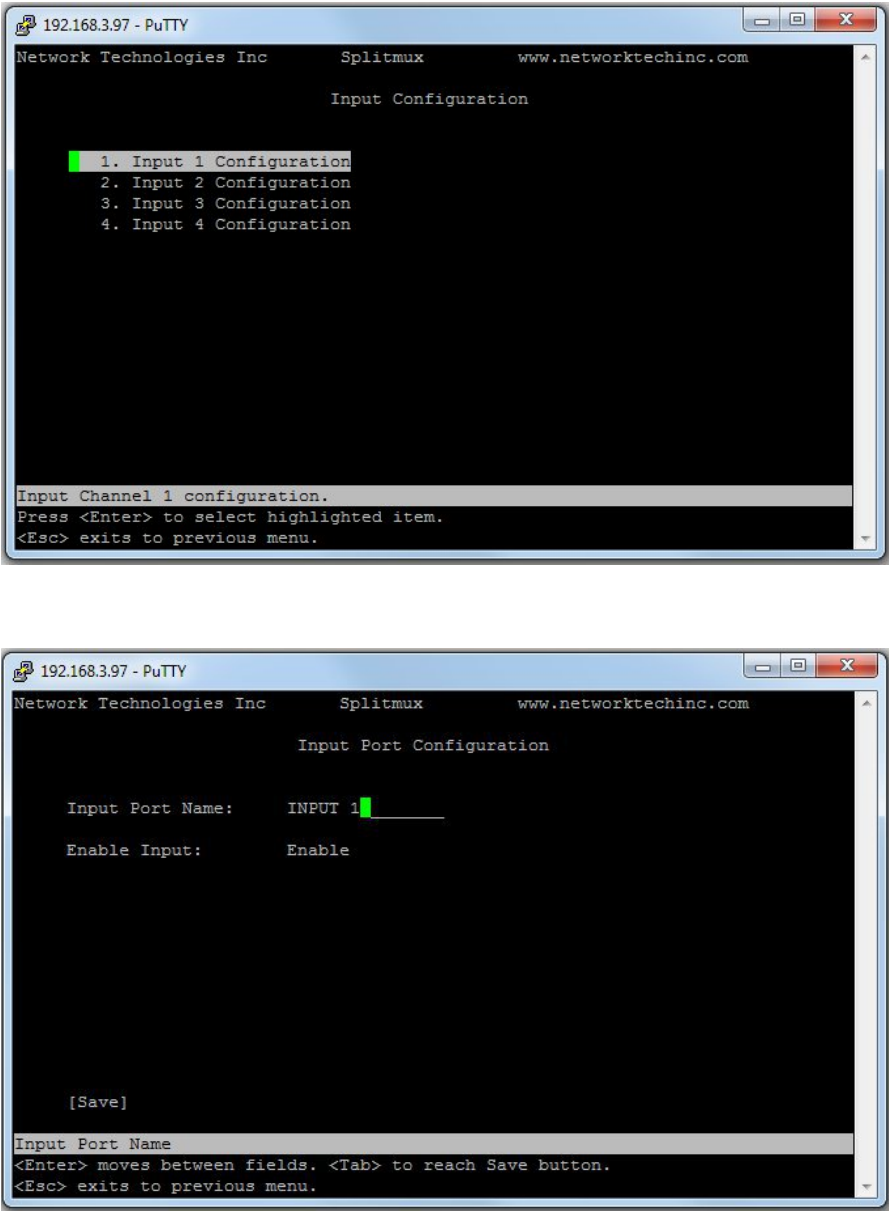
Figure 63- Text Menu- Input Configuration
