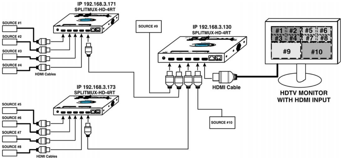
Figure 44- Cascading SPLITMUXs
