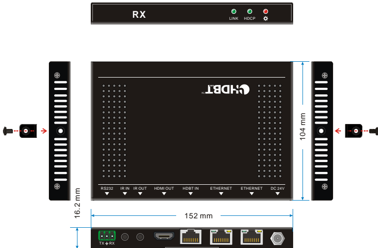
5-2 TPUH422R Receiver
