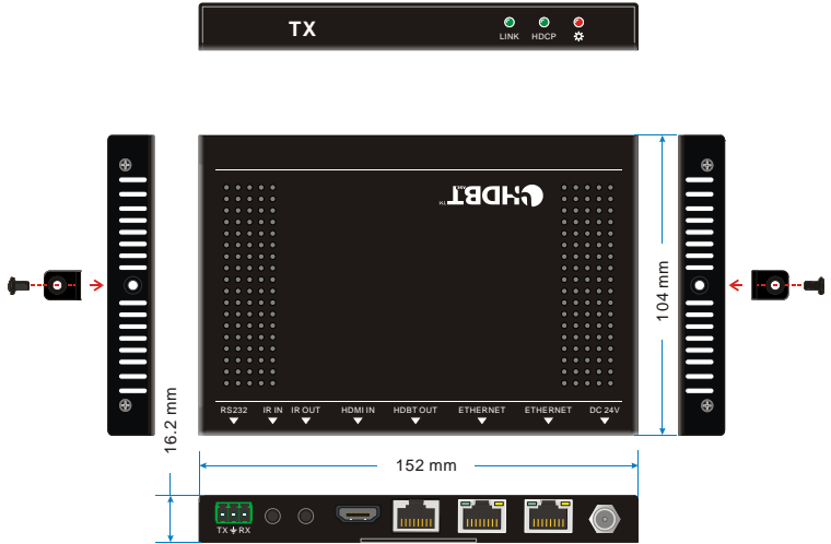
5-1 TPUH422T Transmitter
