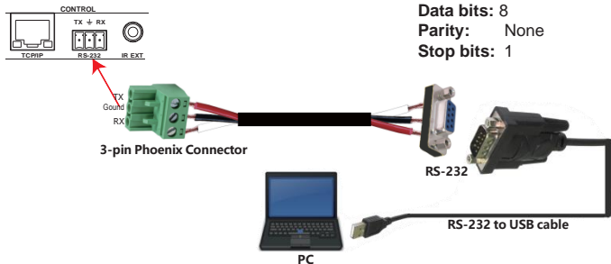
Figure 1: 3-pin phoenix connector to USB
