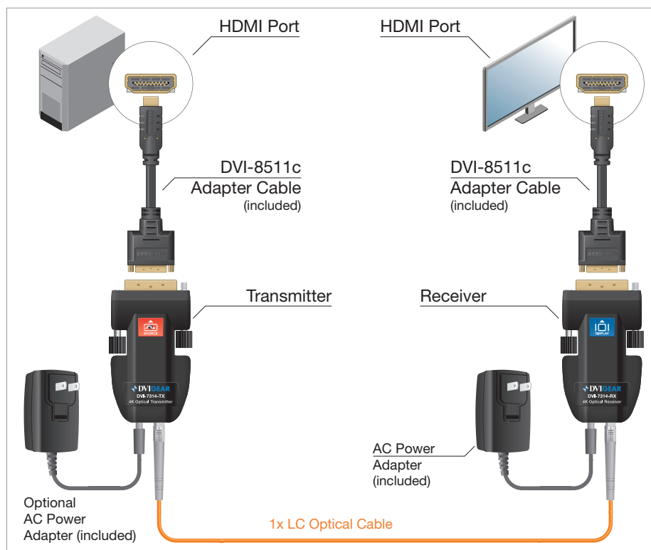
DVI-7313 / DVI-7314 4K Fiber Optic Extenders, 1x LC
