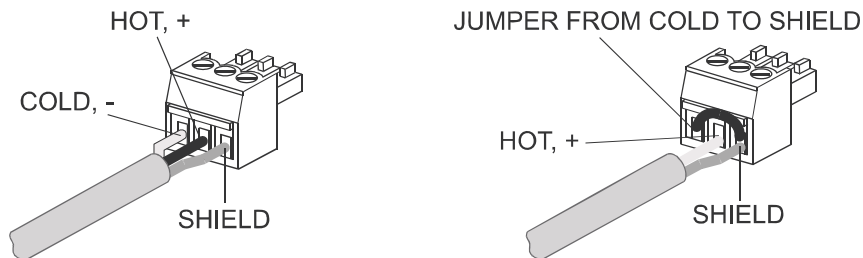
Figure 6.9: Balanced/unbalanced connection of input
