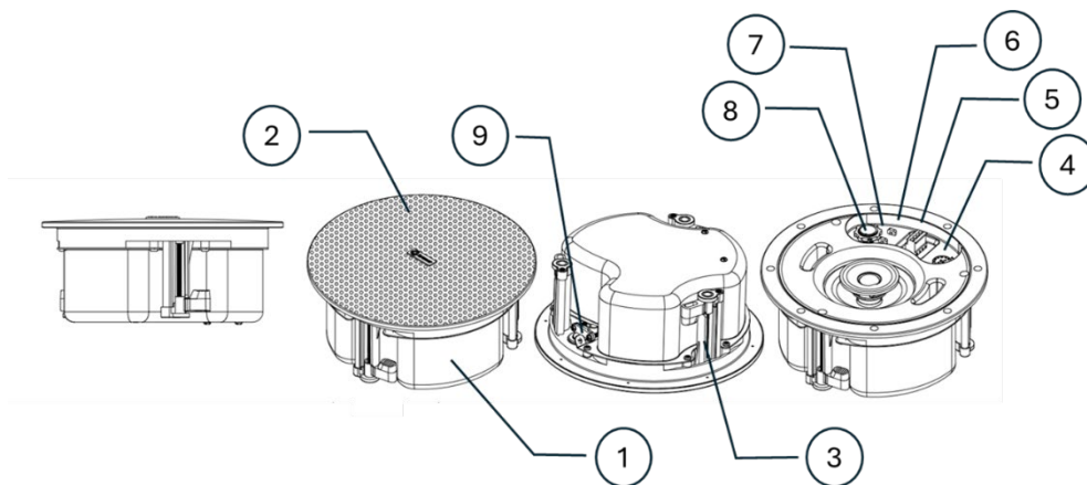
Figure 1 - CL-4P Speaker
