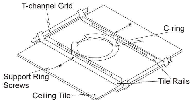
Figure 2 - Mounting the CL-4P in a suspended acoustic ceiling grid
