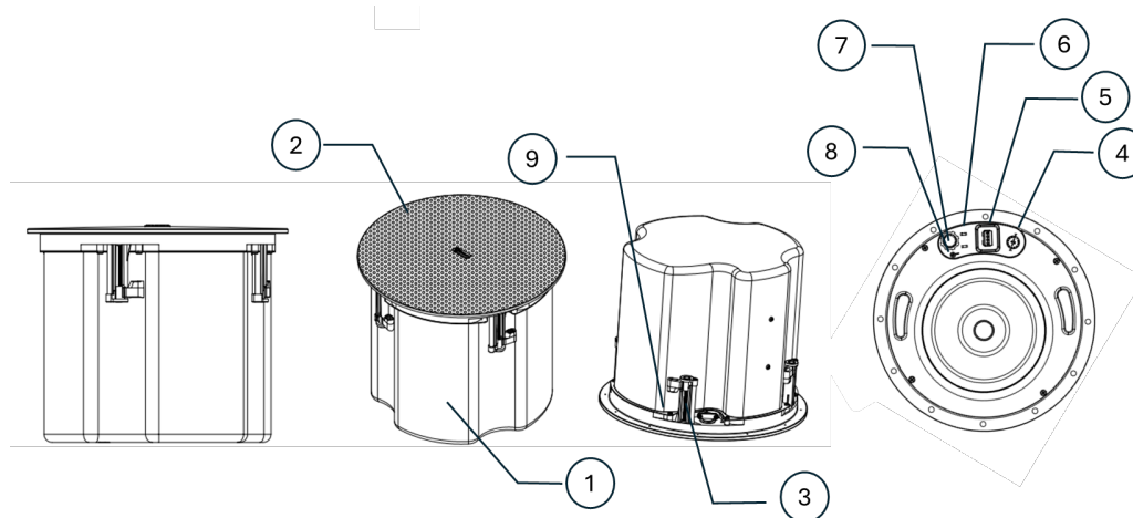
Figure 1 - CL-8P Speaker
