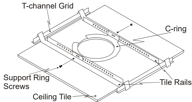
Figure 2 - Mounting the CL-8P in a suspended acoustic ceiling grid
