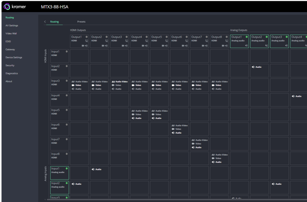
Figure 12: Switching Page with Navigation List on Left
