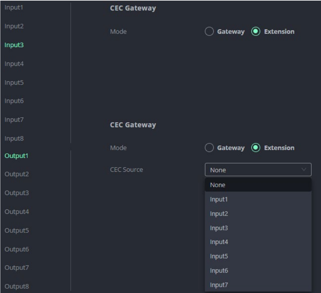
Figure 45: Select Extension Mode for Input/Output Ports
