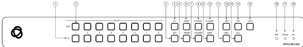
Figure 1: MTX3-88-HSA 4K HDMI 8x8 Matrix Switcher Front Panel
