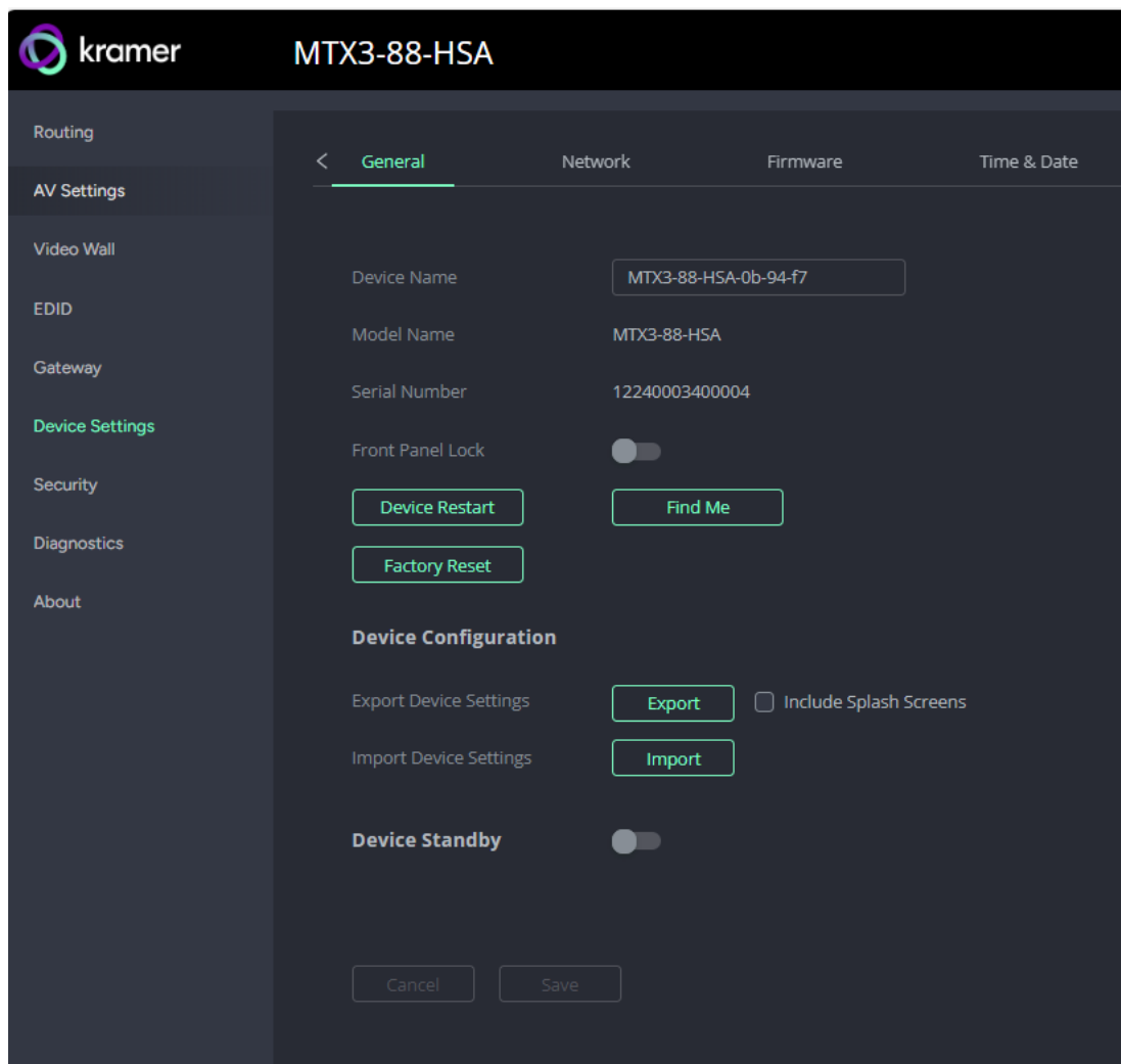
Figure 46: Device > General Page
