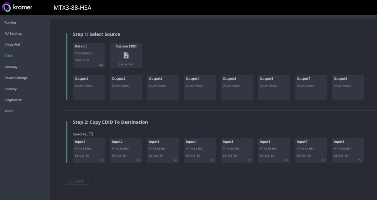
Figure 42: EDID Management Page
