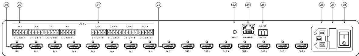
Figure 2: MTX3-88-HSA 4K HDMI 8x8 Matrix Switcher Rear Panel
