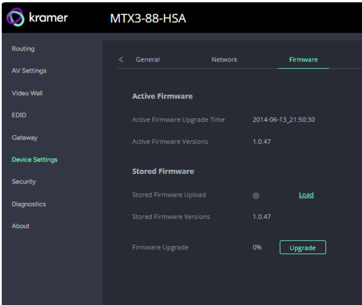
Figure 49: Device Settings &gt; Firmware Page
