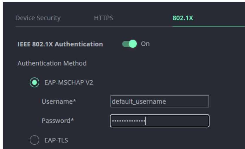
Figure 58: Security Tab – EAP-MSCHAP V2 Authentication
