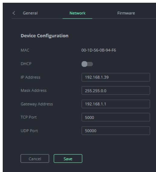
Figure 48: Device Settings > Network Page (DHCP Off)
