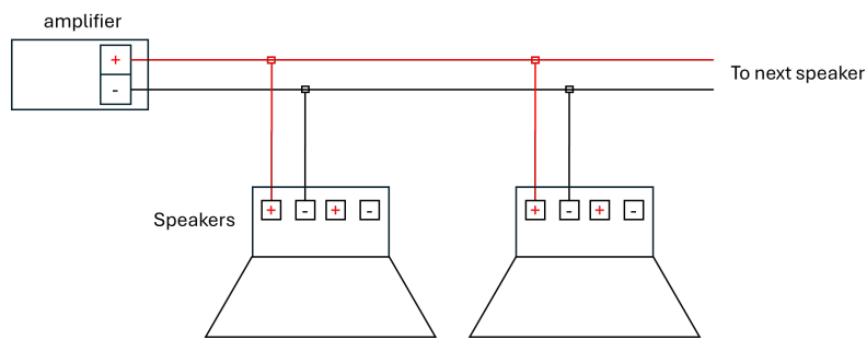
Figure 2 - Parallel Wiring
