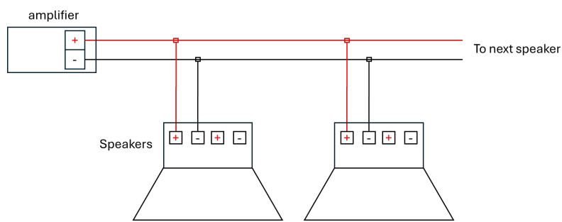
Figure 3 - Parallel Wiring
