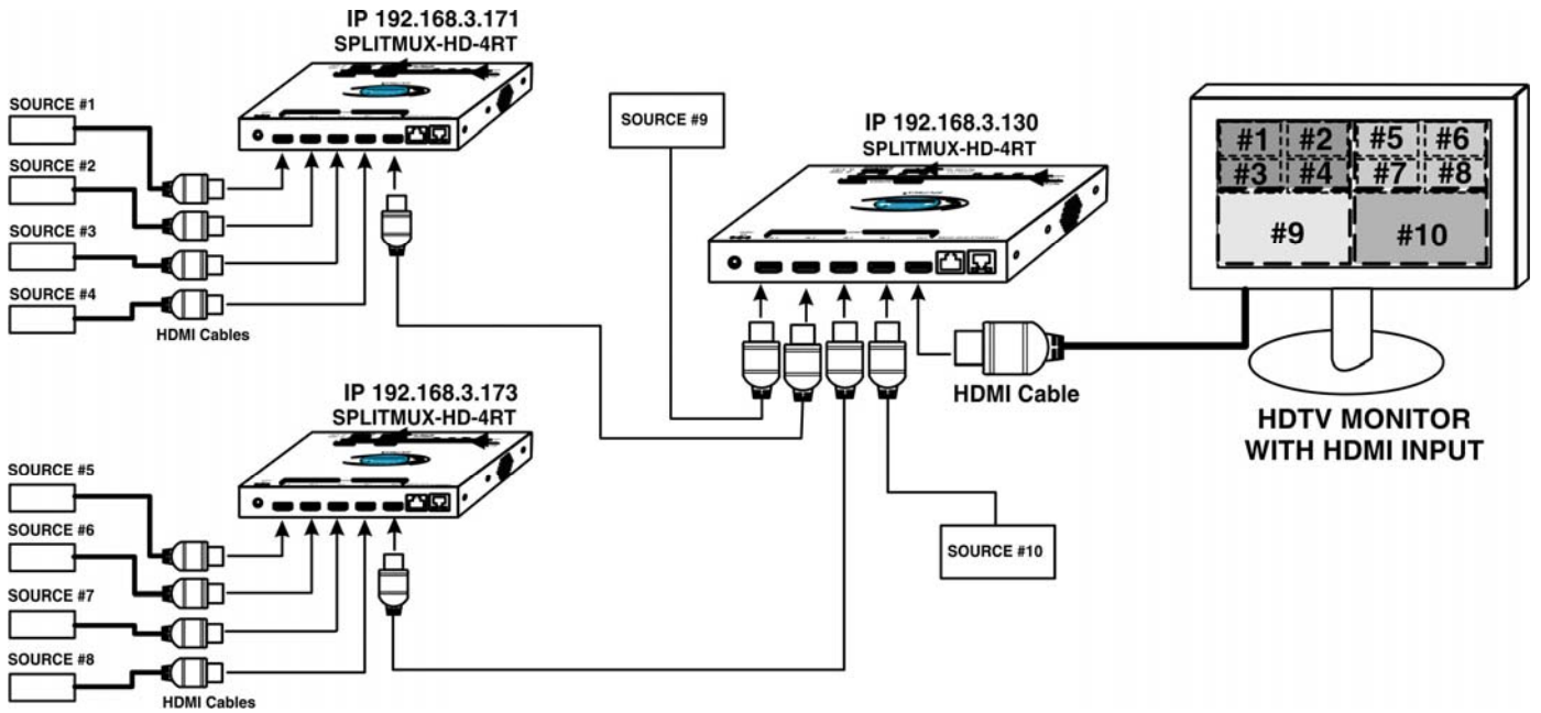
Figure 31- Cascading SPLITMUXs
