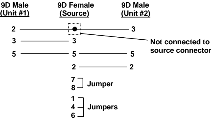
Figure 46- Pinout of Matrix-Y-1 cable
